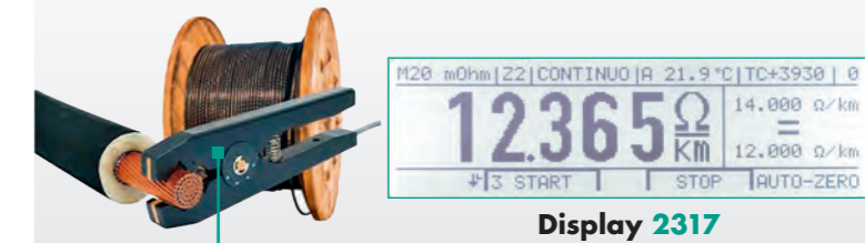
KELVIN test tong 2386-V001 - 4 wire
